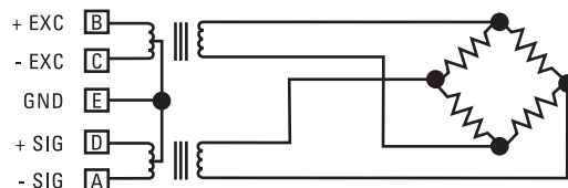
Figure 52. Series 4100 Rotary Transformer Torque Sensor Wiring Code
