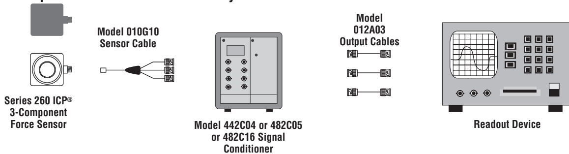
Figure 42. System Utilizing an ICP® Sensor Signal Conditioner
