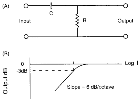
Figure 15. Transfer Characteristics of an ICP® Sensor
