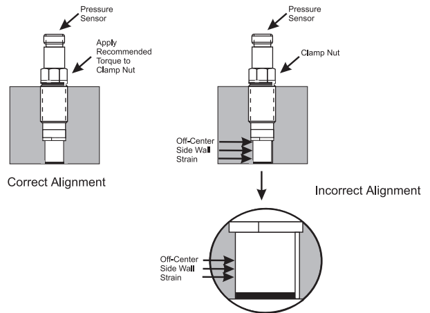
Figure 34. Flush Mount Pressure Alignment
