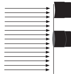
Figure 27. Sound Field Measured by a Pressure Microphone
