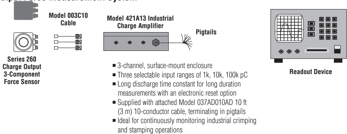
Figure 43. Low-cost System Utilizing 3-Channel Industrial Charge Amplifier
