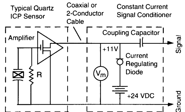
Figure 7. Typical ICP ® Sensor System
