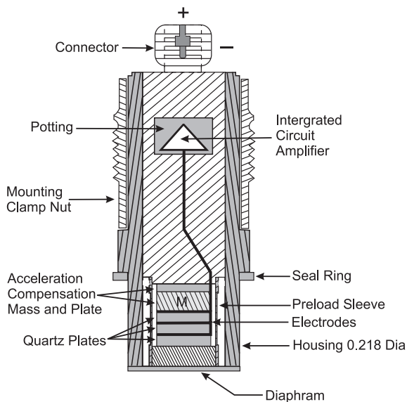
Figure 32. Typical ICP Quartz Pressure Sensor
