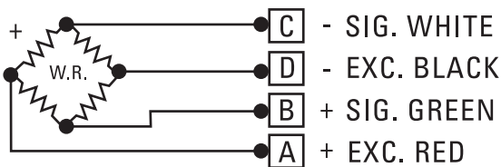
Figure 48. Load Cell Wiring Code
