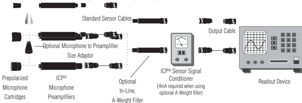
Figure 30. Prepolarized Microphone System
