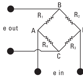
Figure 50. Wheatstone Bridge
