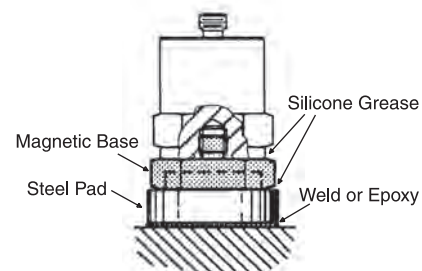
Figure 24. Magnet Mounted to Steel Pad
