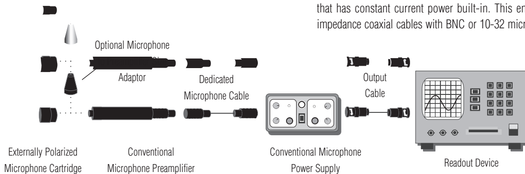
Figure 29. Externally Polarized Microphone System
