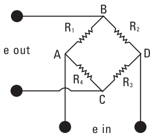
Figure 47. Wheatstone Bridge
