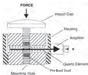
Figure 36. Compression-Tension-Impact Series 208
