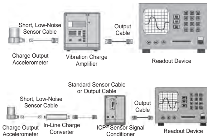
A fixed in-line charge converter may be utilized to simplify setup or to make use of an existing ICP® sensor signal conditioner.
