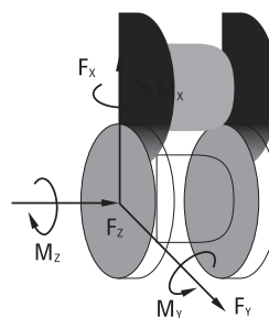
Figure 53. Right-handed Orthogonal Coordinate System
