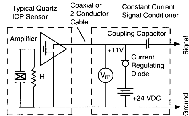
Figure 44. ICP® Sensor System Schematic
