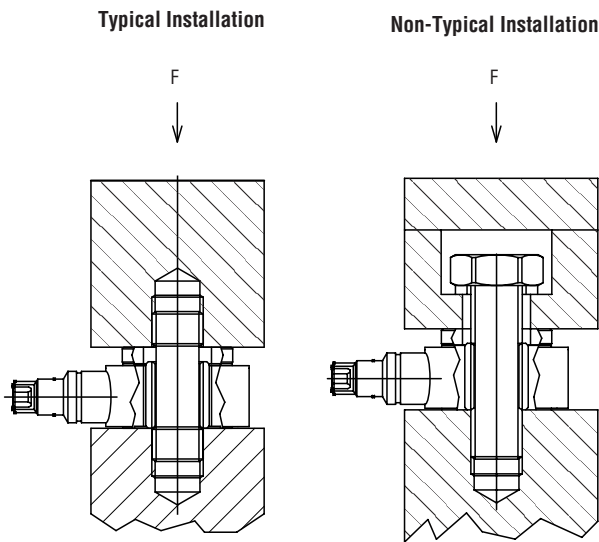
Figure 39. Force Ring Sensor Installations
