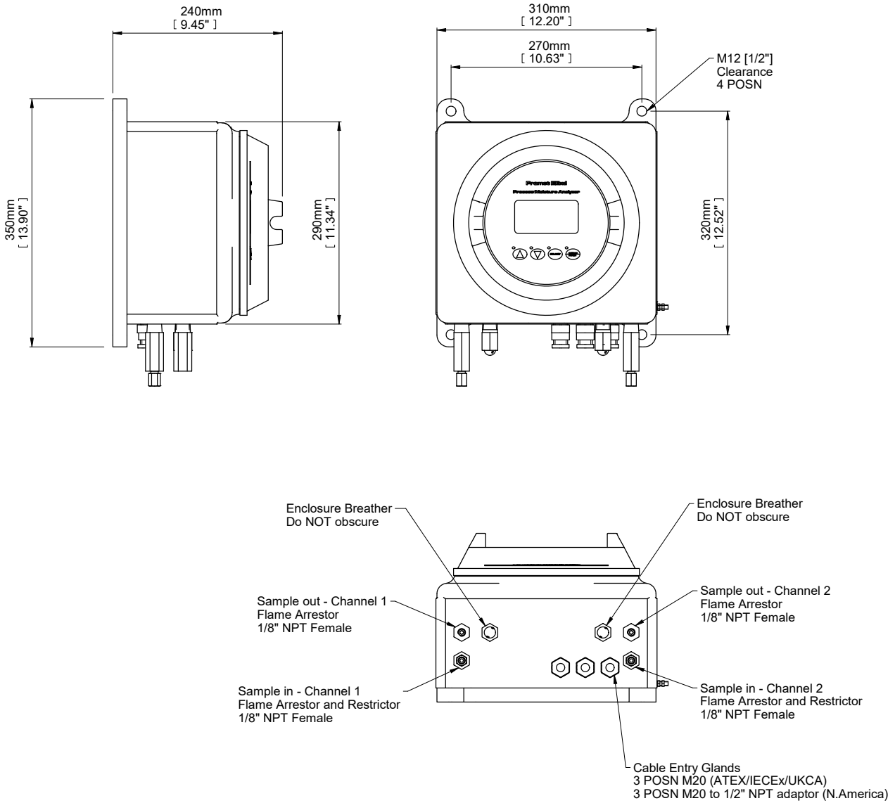
Figure 27 Mounting Drawing
