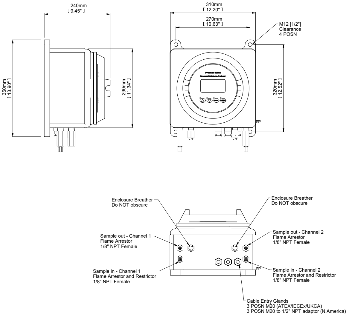
Figure 4 Promet EExd Mounting Drawing
