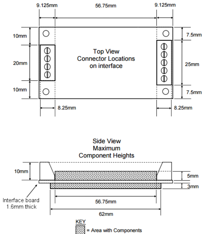
Figure 4-1 - OXY-LC Dimensions
