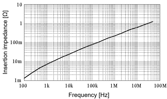
Insertion Impedance (Typical)
