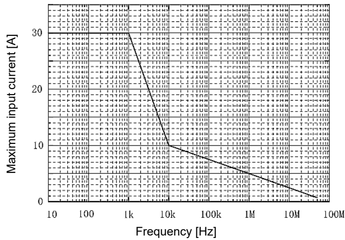
Derating According to Frequency
