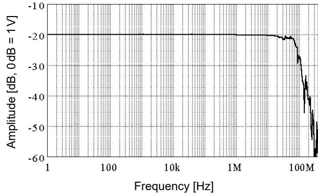
Frequency Response (Typical)
