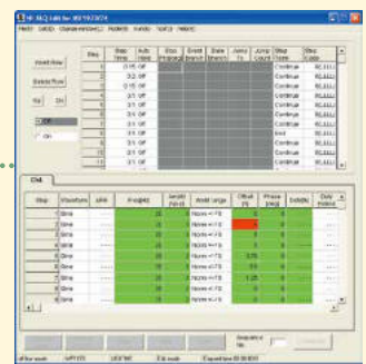
Sequence Editor
