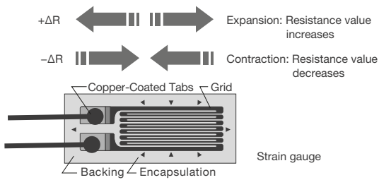
Strain gauge
