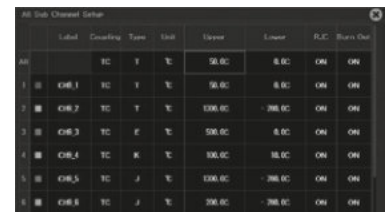
Channel setting screen (DL950)
