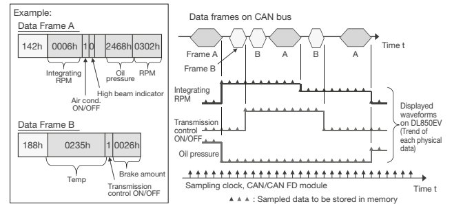
Relationship between sampling data and displayed waveforms, an example
