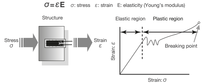
Relationship between strain and stress
