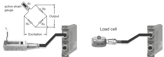
For strain measurements with a strain gauge, use the accessory bridge head.
