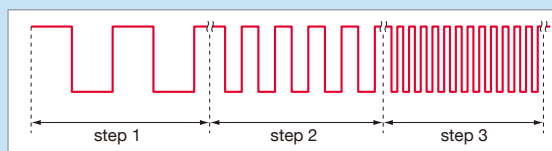
Ex.1 Relay Operation Test (Withstand Power Supply Fluctuation Test)
