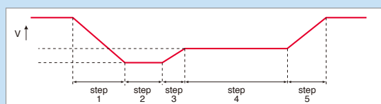
Ex.2 Vehicle Electrical and Electronic Components Test (ISO / DIS7637-2.2 Pulse 4) (Simulation of Transient Voltage Drops at Startup)
