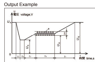
ISO 16750-2 Supply Voltage profile
