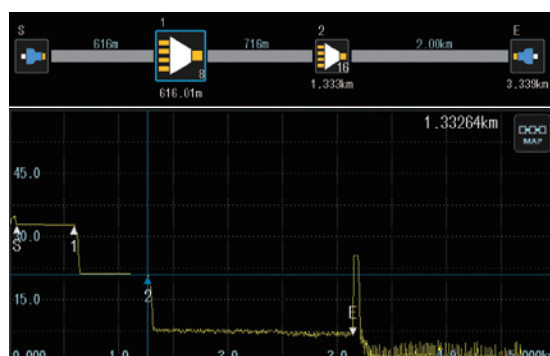
Measurement example of 128-branch splitter
